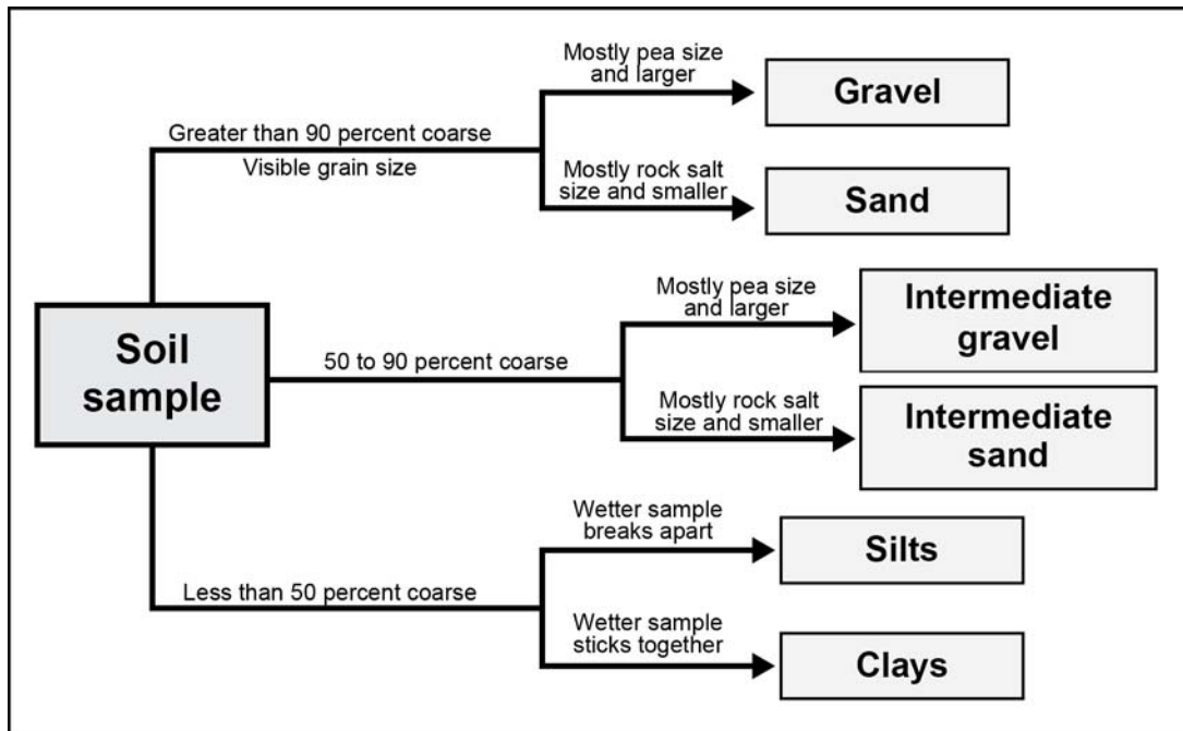
Figure G-18. Soil identification flowchart
