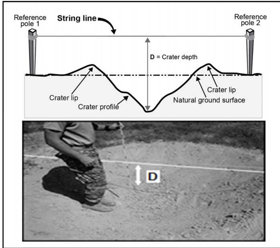
Figure G-15. Step 8. Measure for D
