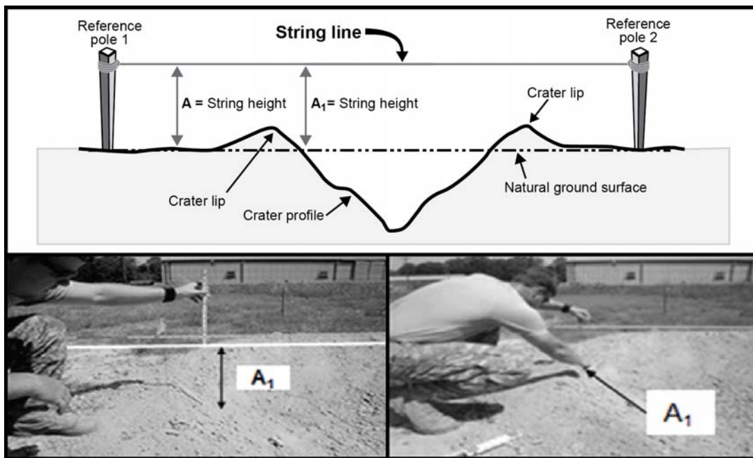
Figure G-12. Step 5. Measure for A_1
