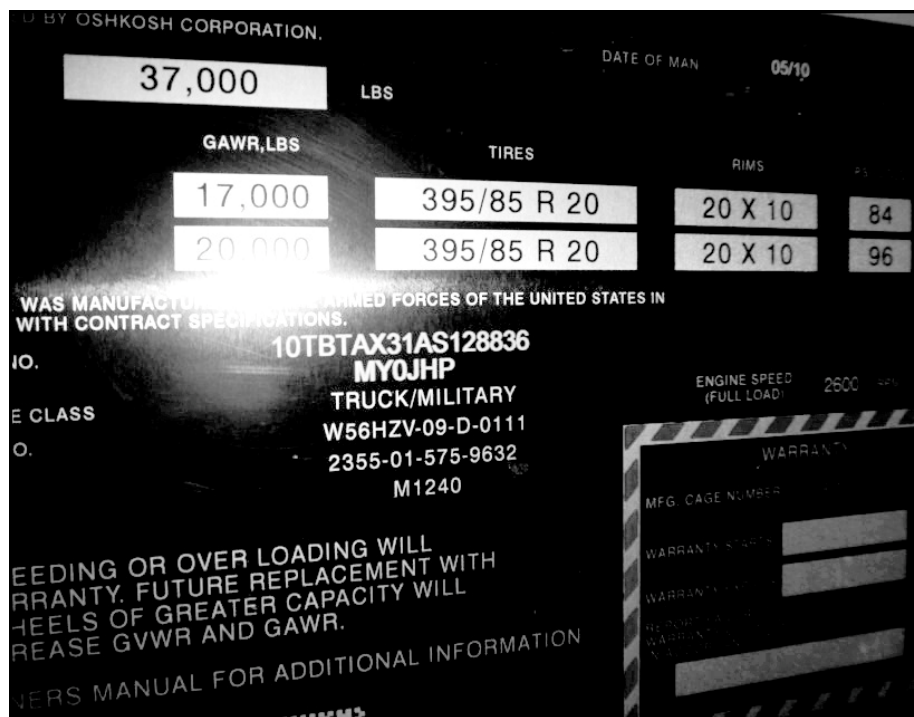
Figure G-28. Vehicle data plate photograph
