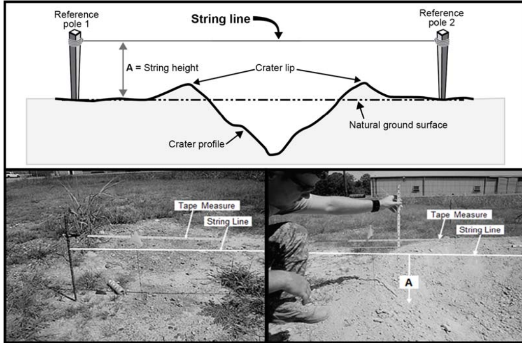
Figure G-10. Step 3. Measure for A
