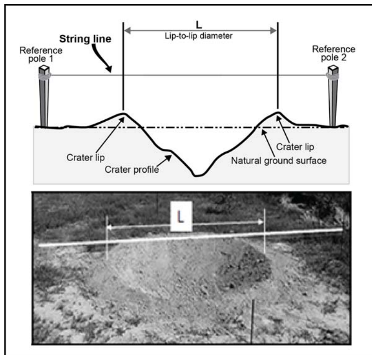
Figure G-14. Step 7. Measure for L
