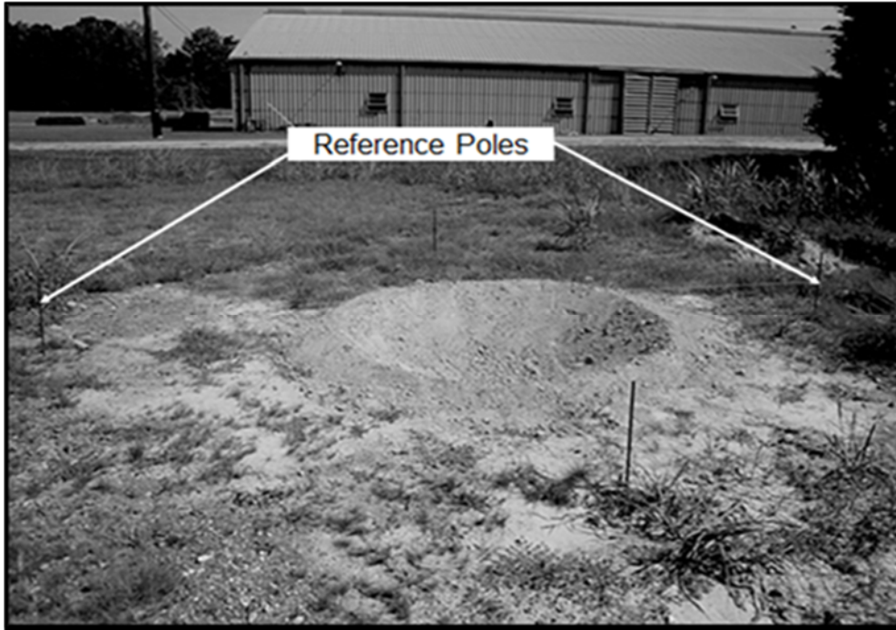
Figure G-8. Step 1. Establish crater dimensions
