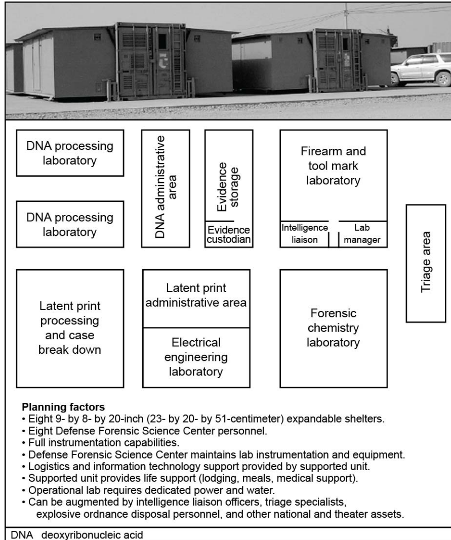
Figure E-1. Forensic exploitation team lite forensic laboratory
