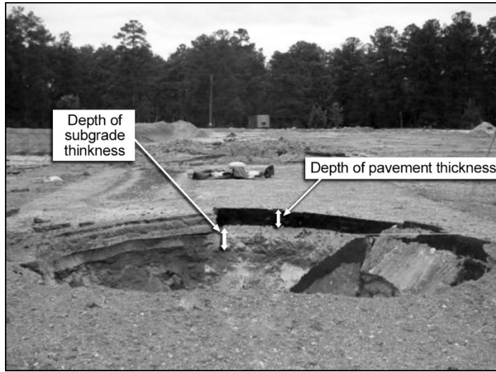
Figure G-6. Pavement measurements
