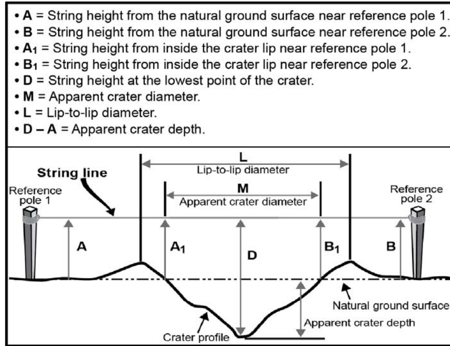
Figure G-4. Critical crater measurement checklist
