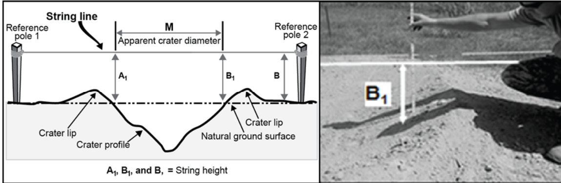
Figure G-13. Step 6. Measure for B_1
