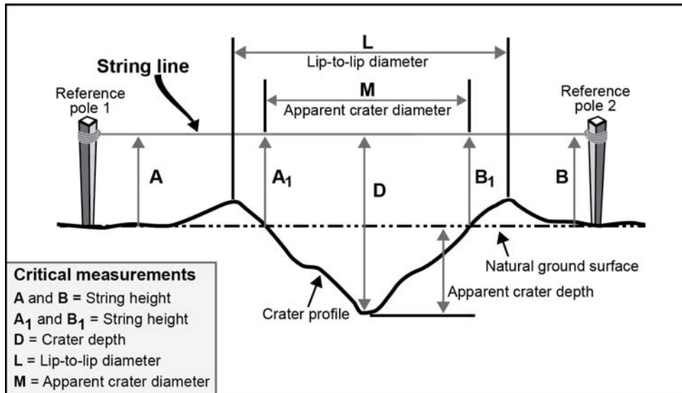
Figure G-7. Expedient crater measurements
