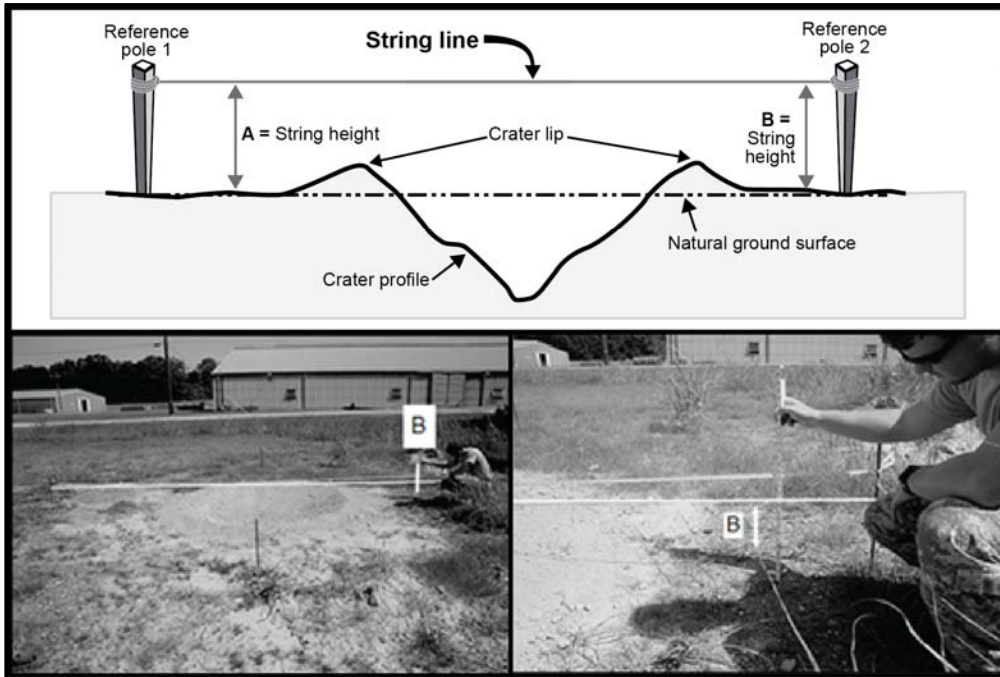
Figure G-11. Step 4. Measure for B
